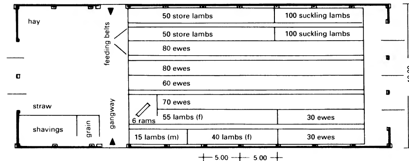
10 Sheep shed for 350 ewes, 110 lambs and 200 suckling lambs, 100 store lambs
